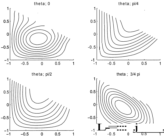
Figure 9. First eigenmode for different lamination angles (II case)
