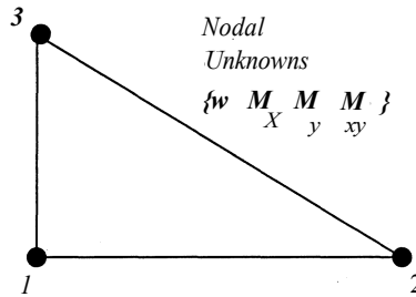
Figure 1. The triangular finite element used in the numerical examples
