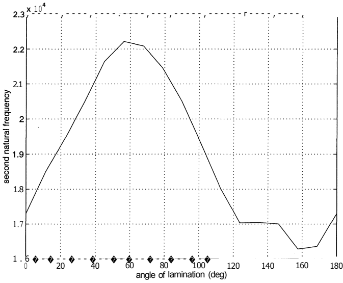
Figure 7. Second natural frequency for different lamination angles (I case)
