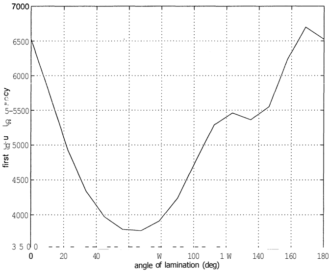
Figure 12. First natural frequency for different lamination angles (II case)
