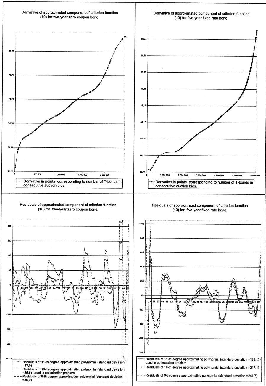
Figure 2. Derivatives and residuals of approximated components of criterion function for T-bonds
